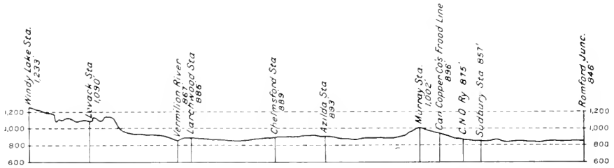
Fig. 3.—Section from Romford Junction, near Sudbury, Ontario, to Windy Lake, along the main line of the Canadian Pacific Railway. This section crosses the Sudbury basin and shows the elevations above sea level along the railway track. Horizontal scale 8 miles equals 1 inch; vertical scale 1,600 feet equals 1 inch.
